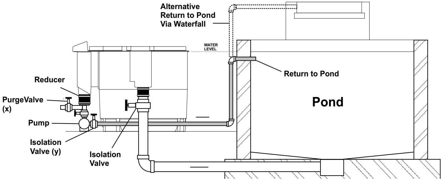
Fig. 8 - A Typical Gravity Fed System
